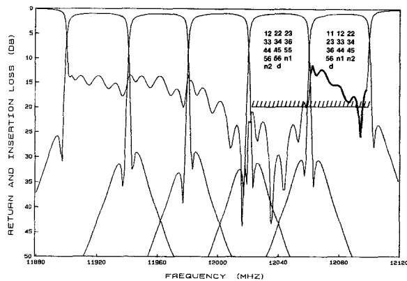
Fig. 2(d) Responses after the third suboptimization
